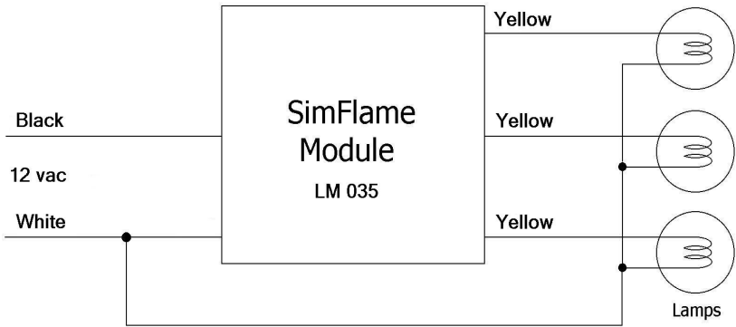
Wiring Diagram
