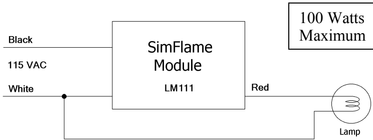
Wiring Diagram
