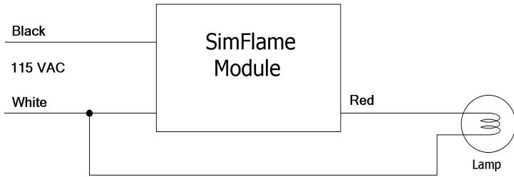
Wiring Diagram
